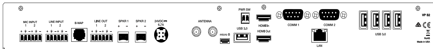
Audio Presenter HUB Back Panel
