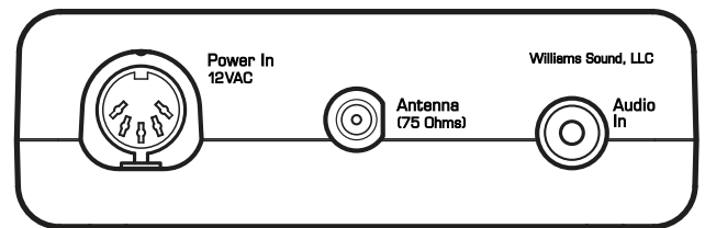
PPA T27 Rear Panel:
