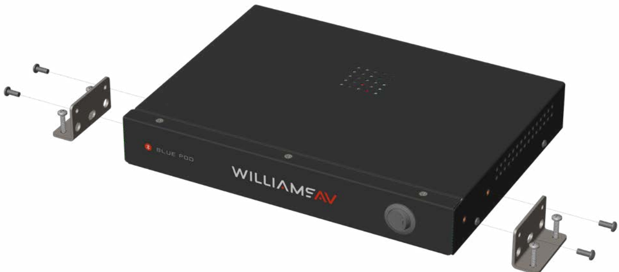
Figure 2: Insert the screws as shown for mounting on top of a surface.
