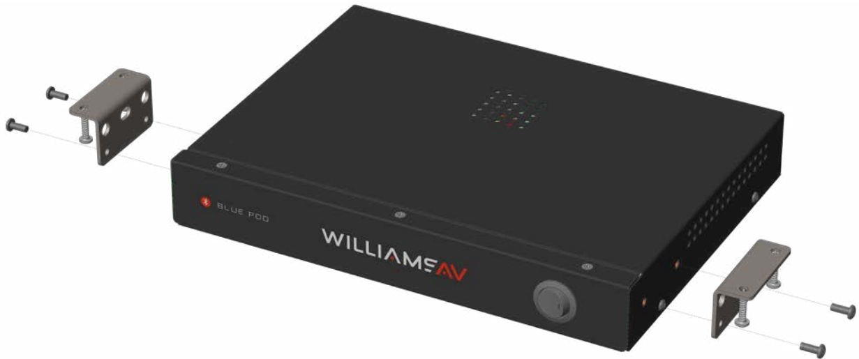
Figure 3: Insert the screws as shown for mounting underneath a surface.
